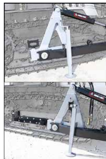
Sgancio rapido Quick coupling/uncoupling system
